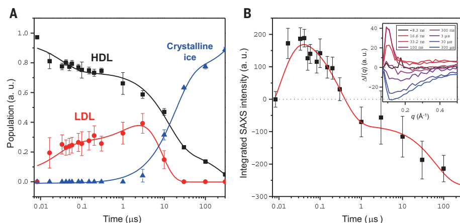
Fig. 4. Time-dependent population changes and SAXS intensity. (A) Time-dependent population changes of HDL (black squares), LDL (red circles), and crystalline ice (blue triangles). The solid black, red, and blue lines are shown to guide the eye. The error bar at each data point indicates the standard error determined from 20 independent measurements. (B) Time-dependent integrated SAXS intensity from q = 0.1 to 0.3 \text{ \AA}^{-1} . The solid red line is shown to guide the eye. (Inset) The difference between the unpumped and pumped scattering curves at various time delays in the SAXS region. After 1 \mu\text{s} , the samples became more homogeneous than the unpumped sample, resulting in a negative SAXS difference.
